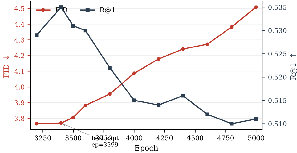
Figure 4: EgoPed training trajectory: training-time validation FID (left axis, red) and R@1 (right axis, blue) across the late training segment. Epoch 3399 is the best checkpoint (highest R@1, FID within noise of epoch 3199, and best definitive 3-replication FID); both metrics then degrade steadily through epoch 4999. Training loss is flat across this range — sampling quality oscillates independently of training loss.
