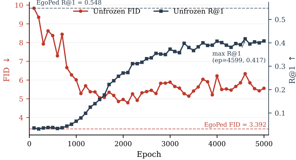
Figure 3: Unfrozen training trajectory: training-time validation FID (left axis, red) and R@1 (right axis, blue) vs. epoch, over the full 5000-epoch run. FID is best at epoch 2099 and degrades as R@1 rises; after epoch \approx 3299 , R@1 saturates in the 0.37–0.42 band while FID oscillates between 5.1 and 6.3. Dashed reference lines show EgoPed’s best operating point (FID=3.392, R@1=0.548 at epoch 3399, CFG 10). Unfrozen never approaches EgoPed’s performance on either metric.
