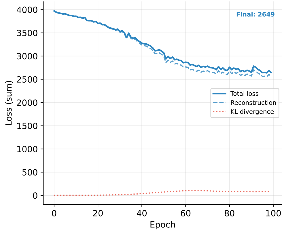
LSTM-VAE Pooled
