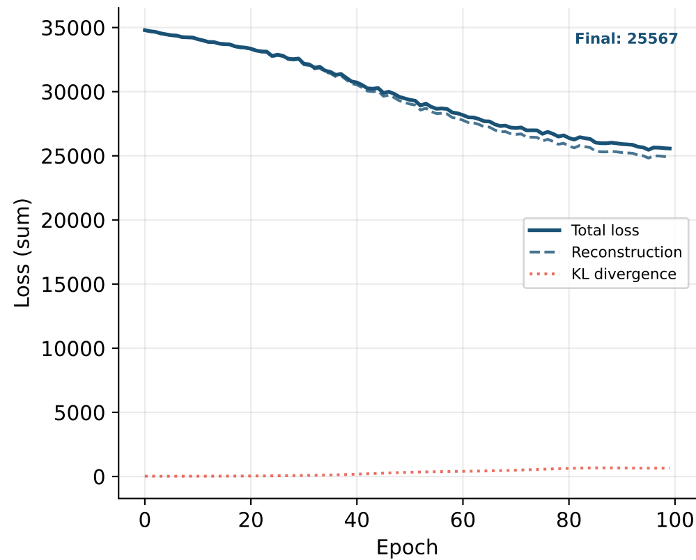
LSTM-VAE Pooled
