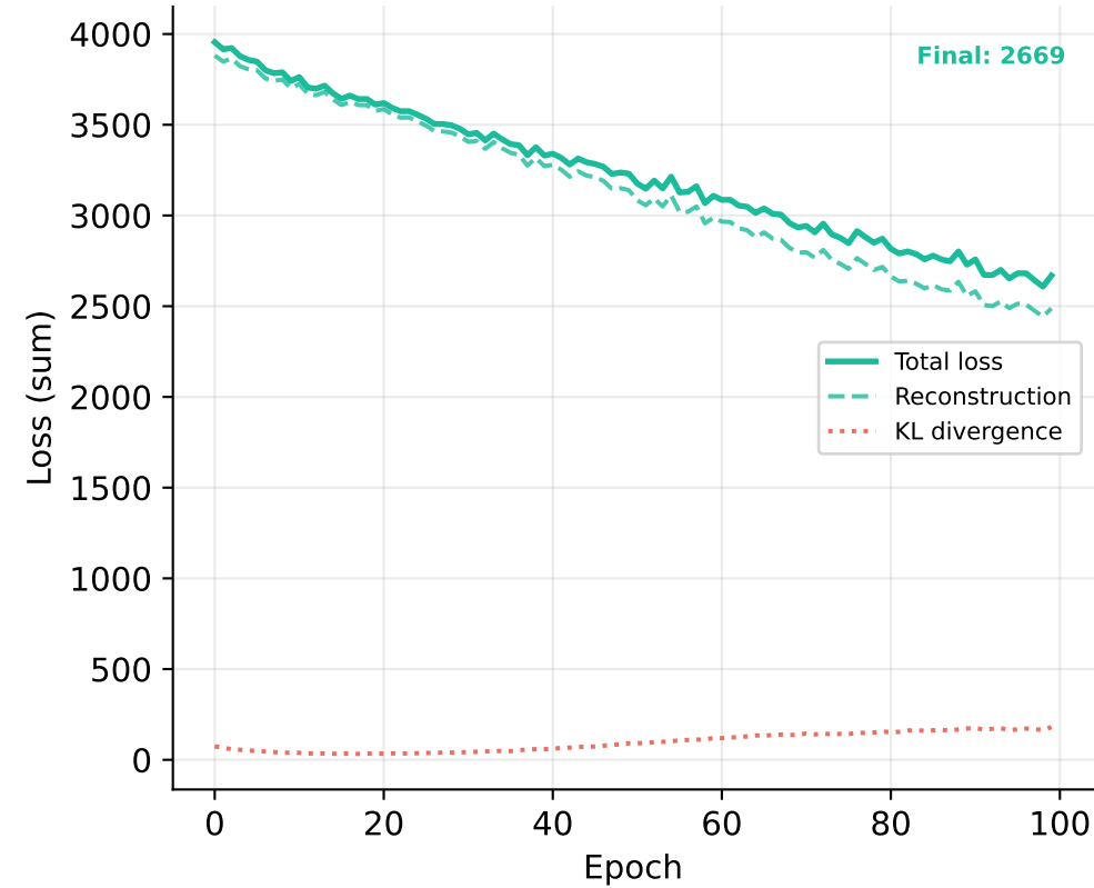
OmniAnomaly Pooled
