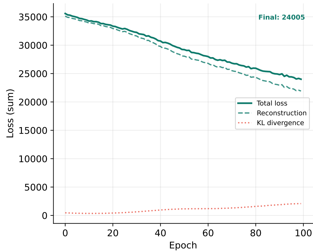
OmniAnomaly Pooled
