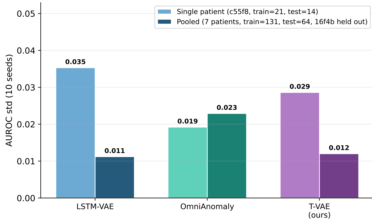
AUROC Stability (↓ = more reproducible)
