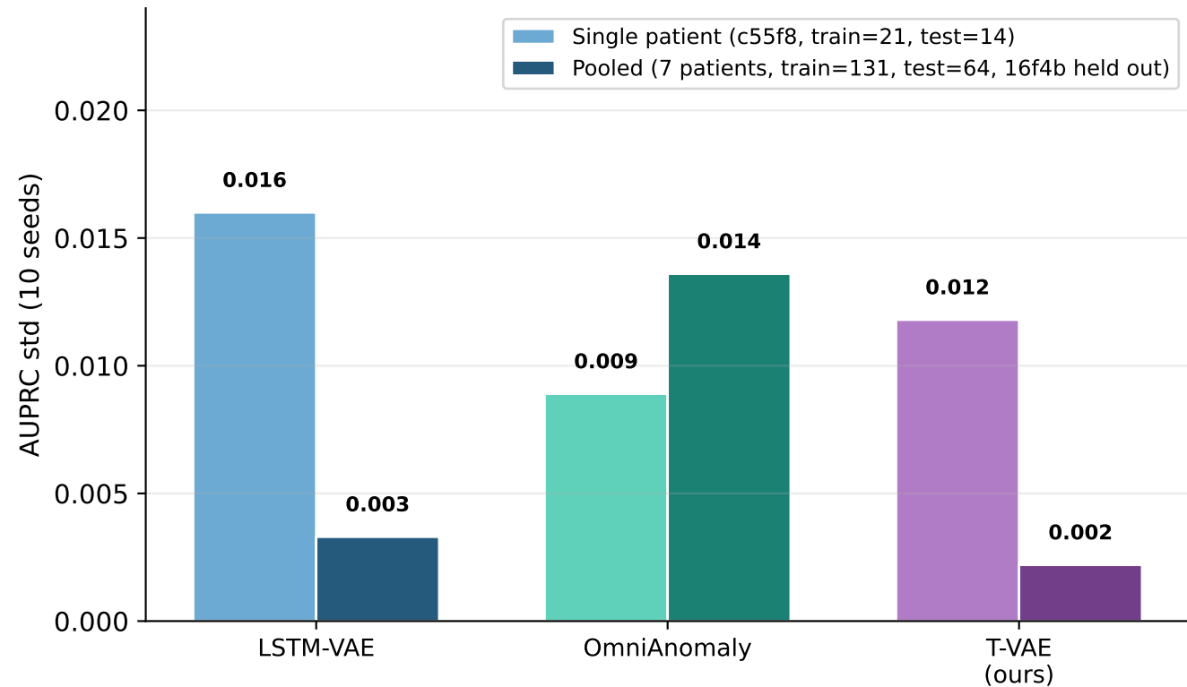
AUPRC Stability (↓ = more reproducible)
