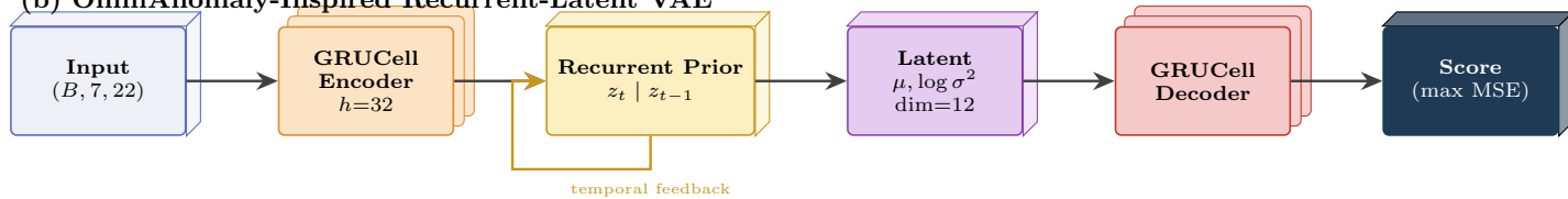
(b) OmniAnomaly-Inspired Recurrent-Latent VAE
