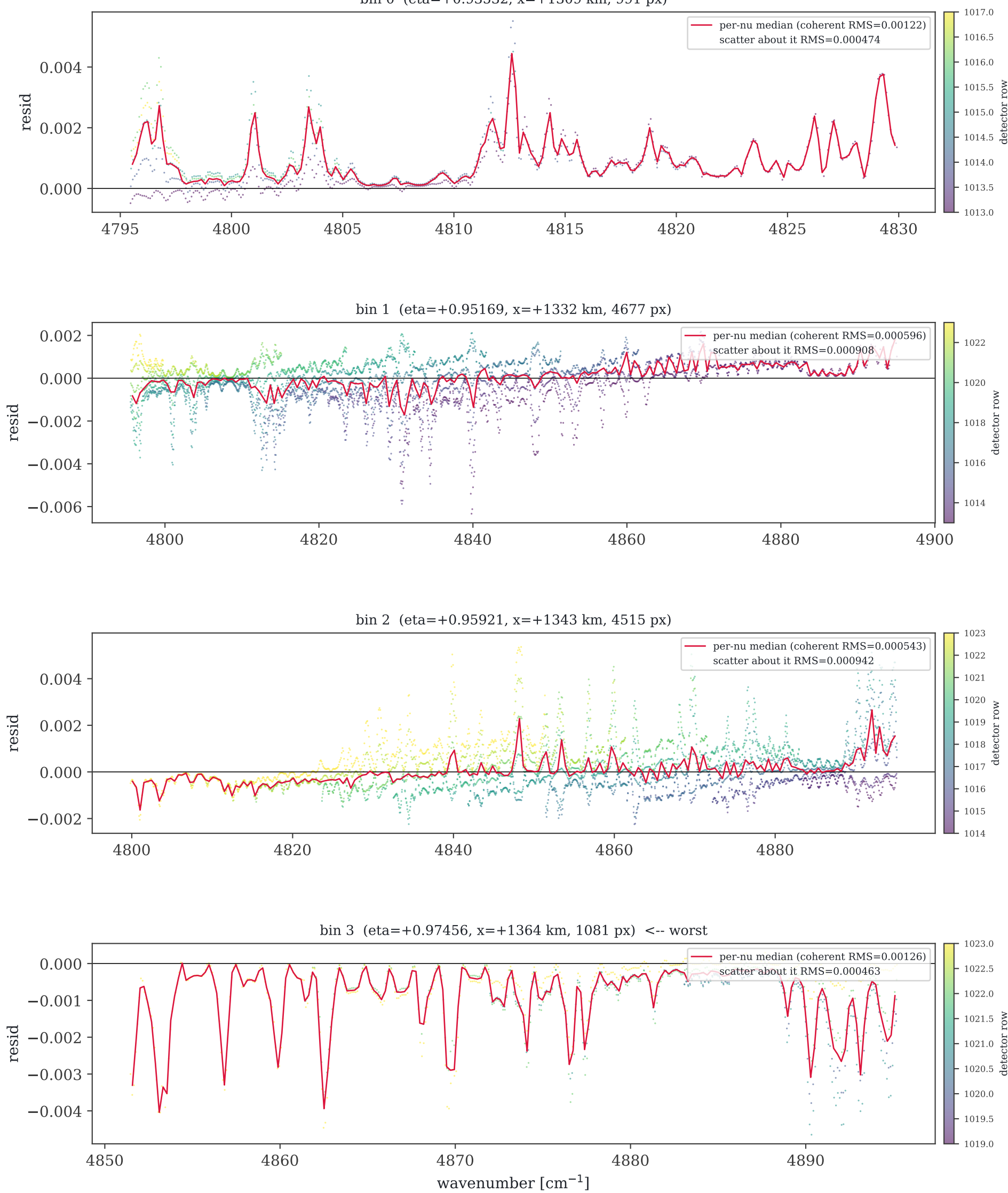
FPA2 joint block rows 1013-1023 -- residual in FITTING space (coarse): within-bin residual vs. wavenumber
