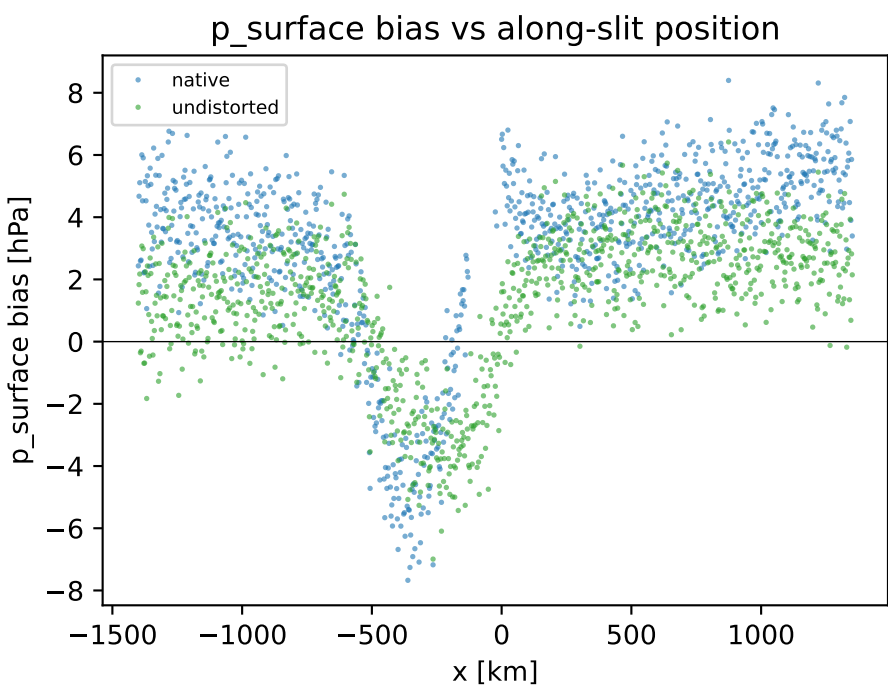
Where each pipeline fails, vs along-slit position
