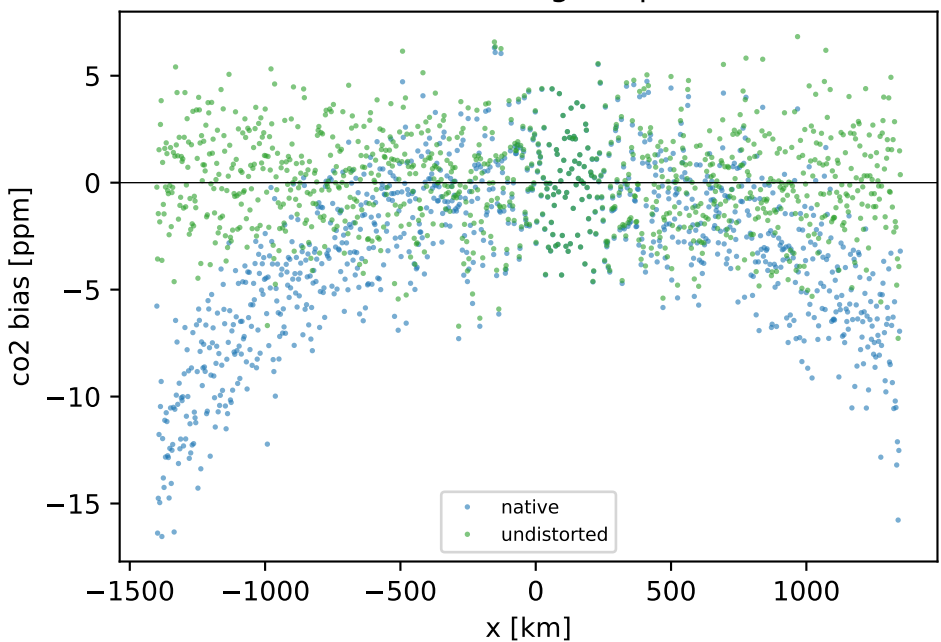
co2 bias vs along-slit position
