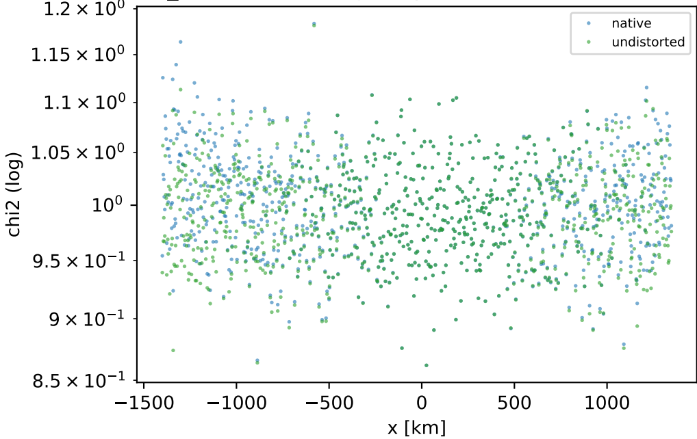
chi2_reduced vs along-slit position (outliers excluded)
