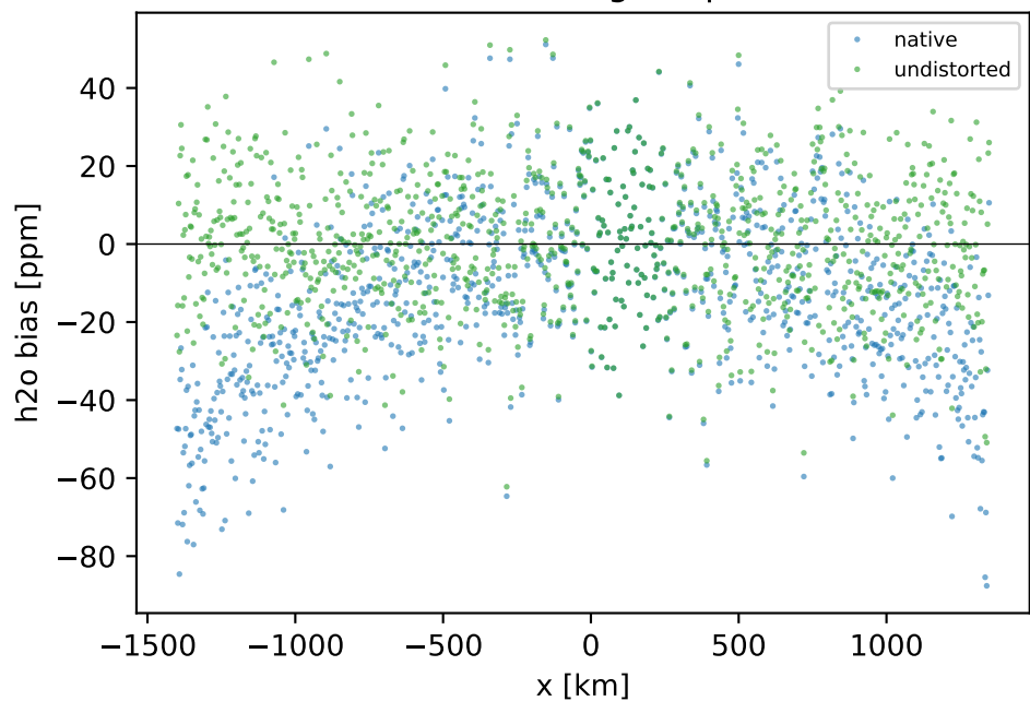
h2o bias vs along-slit position
