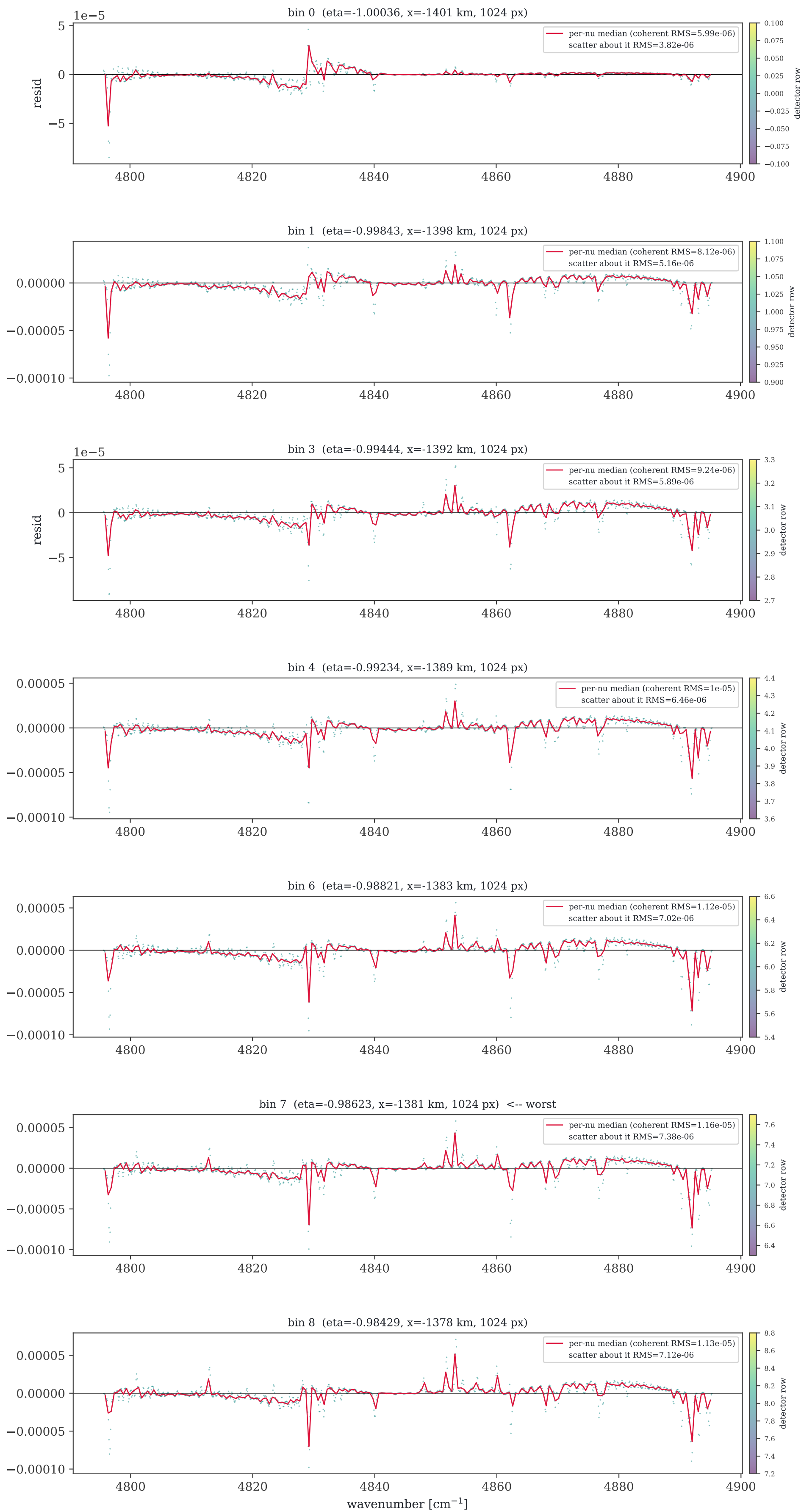
FPA2 joint block rows 0-8 -- residual in FITTING space (hires): within-bin residual vs. wavenumber
