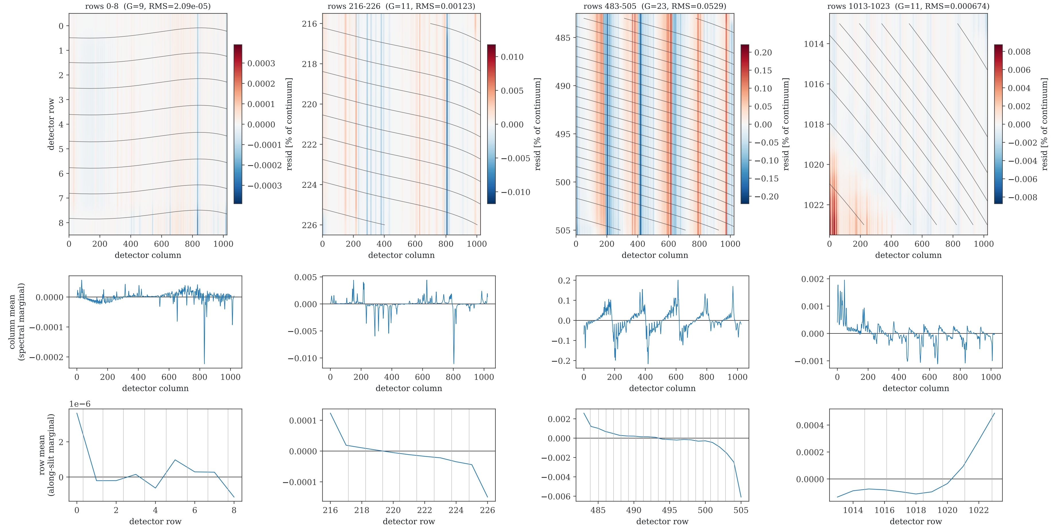
FPA2 joint block -- post-fit residual in DETECTOR space (hires; grey lines = eta bin edges)
