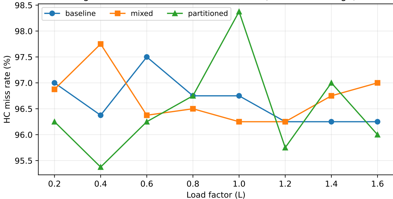
Fig.3: Baseline vs Mixed vs Partitioned (Wide Load Range)
