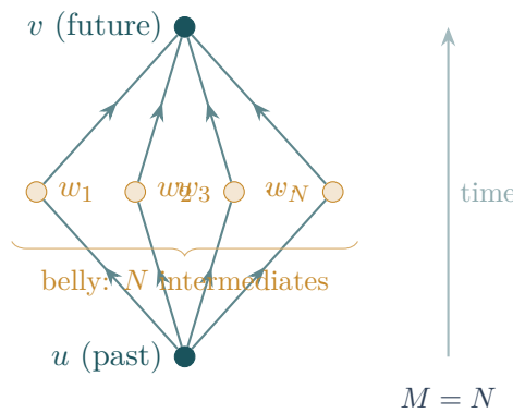
Figure 11.1: The Causal Prism K_{2,N} . Two poles u (past) and v (future) are connected through N mutually disconnected intermediates w_i . Every edge is a directed Hasse link; no intermediate–intermediate edges exist (triangle-freeness). The topological mass is M = N .
