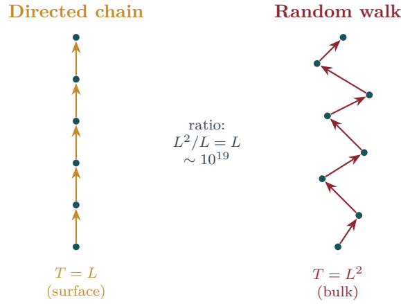
Figure 10.1: The hierarchy mechanism. Left: a directed chain along a prism surface traverses L links in time T = L (gauge forces). Right: a diffusive walk through the 4D bulk requires T = L^2 steps to cover the same distance (gravity). The ratio L^2/L = L \sim 10^{19} explains the 10^{38} -fold hierarchy between gravity and gauge forces without fine-tuning.
