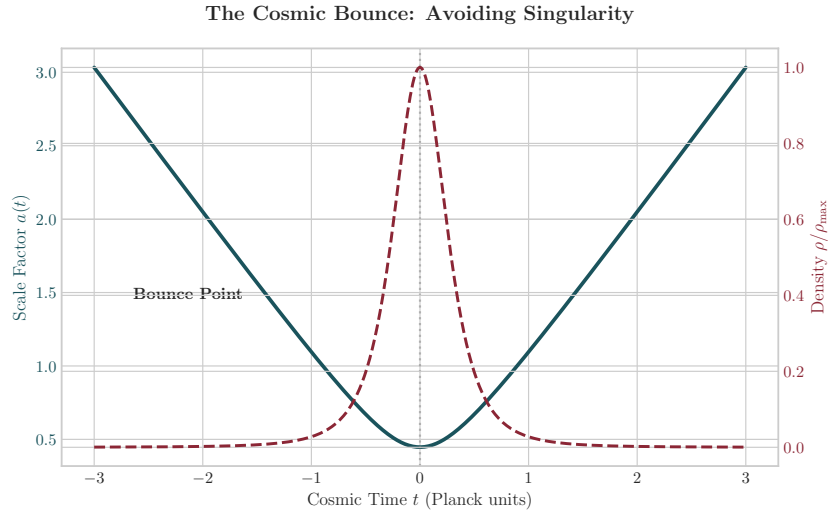
Figure 10.2: The Kuratowski epoch. At maximum density, the causal set is a total order (chain); transitive reduction produces the Hasse diagram; as density drops, spatial width emerges and the first K_5 contractions produce matter (prisms). The Big Bang singularity is replaced by a smooth bounce at \rho = \rho_{\max} .
