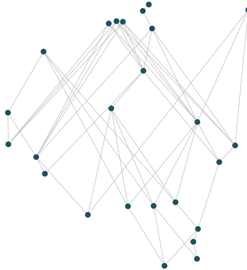
Figure 11.2: A 25-event Hasse diagram generated from a Poisson sprinkling in 1+1D. Each dot is a spacetime event; each line is a covering relation. Causal Prisms K_{2,N} appear wherever two events share multiple intermediates.
