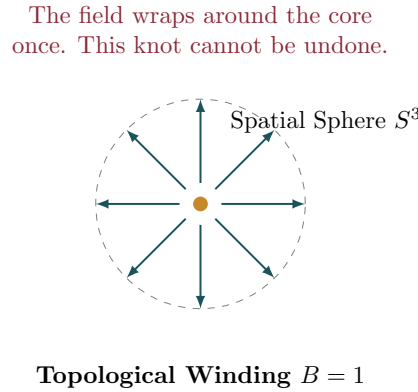
Figure 21.1: The Skyrmion hedgehog configuration with winding number B = 1 . The proton is a topological knot in the causal layer ordering, protected by \pi_3(S^3) = \mathbb{Z} . Un-knotting requires coordinated rearrangement of \sim 10^{60} links, giving \tau_p > 10^{40} yr.
