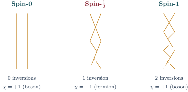
Figure 15.1: Spin as inference braid. Two causal chains through a prism form a braid. No crossings: spin-0 (boson). One crossing (half-twist): spin- \frac{1}{2} (fermion). Two crossings (full twist): spin-1 (boson). The chirality \chi = (-1)^{2s} recovers the spin-statistics theorem.
