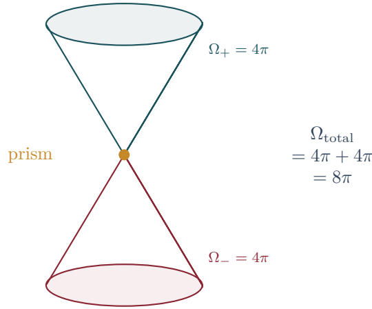
Figure 17.1: Isotropic projection. A Causal Prism radiates into the future light cone ( \Omega_+ = 4\pi ) from the origin pole and receives from the past light cone ( \Omega_- = 4\pi ) at the destination pole. The total interaction solid angle is \Omega = 8\pi , giving \alpha = Q_{\text{topo}}/(8\pi) .
