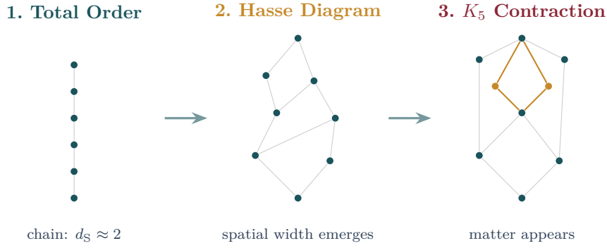
Figure 20.1: The Kuratowski Epoch in three steps. (1) The primordial total order: all events linearly ordered, d_S \approx 2 . (2) Transitive reduction creates the Hasse diagram: spatial width emerges. (3) K_5 contraction freezes topological defects into Causal Prisms (ochre nodes): matter is born.
