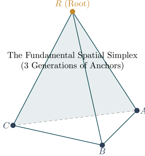
Figure 18.1: The fundamental spatial simplex (tetrahedron). The three anchors of the democratic mass matrix correspond to three equivalent vertices. The eigenvalue structure \{3k, 0, 0\} arises from the S_3 symmetry of the simplex: one coherent superposition (heavy) and two antisymmetric cancellations (light).
