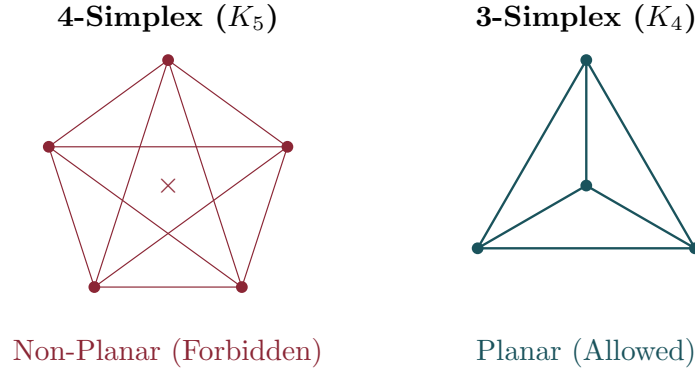
Figure 15.2: Left: the 4-simplex K_5 (non-planar)—forbidden by Kuratowski’s theorem. Right: K_4 (planar but not a Hasse subgraph). Attempting to place two identical fermionic prisms in the same causal neighbourhood forces a K_{3,3} minor, enforcing the Pauli exclusion principle through graph planarity.
