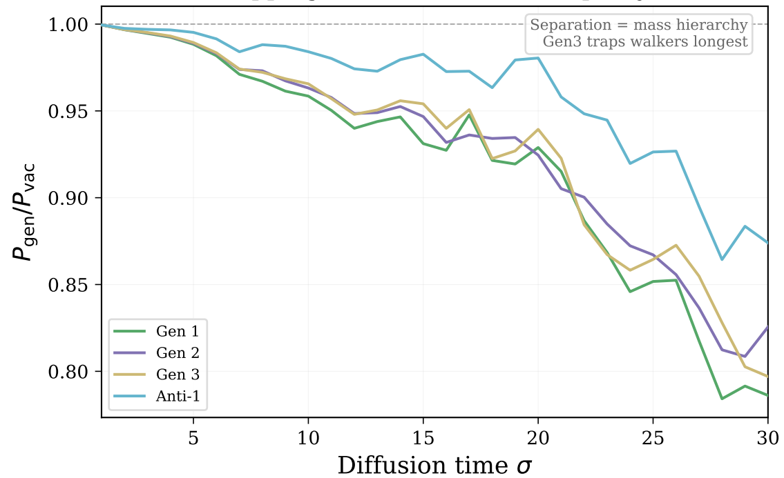
Trapping Enhancement (mass proxy)
