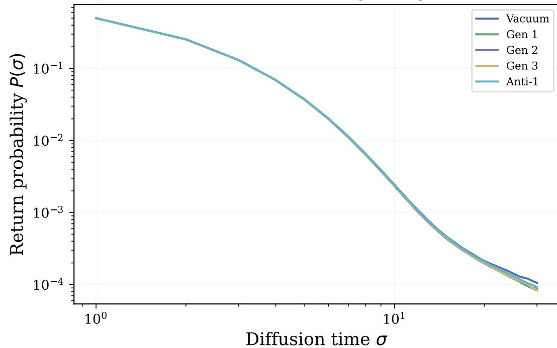
Return Probability Decay
