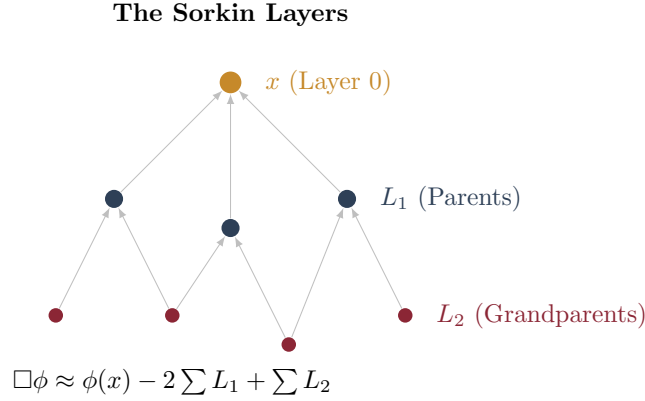
Figure 4.1: The Sorkin Layers. To calculate the d'Alembertian at x , we sum over the field values at layers of ancestors L_1, L_2 , etc. This non-local sampling recovers the local continuum operator.
