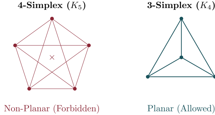
Figure 15.2: Left: the 4-simplex K_5 (non-planar)—forbidden by Kuratowski’s theorem. Right: K_4 (planar but not a Hasse subgraph). Attempting to place two identical fermionic prisms in the same causal neighbourhood forces a K_{3,3} minor, enforcing the Pauli exclusion principle through graph planarity.
