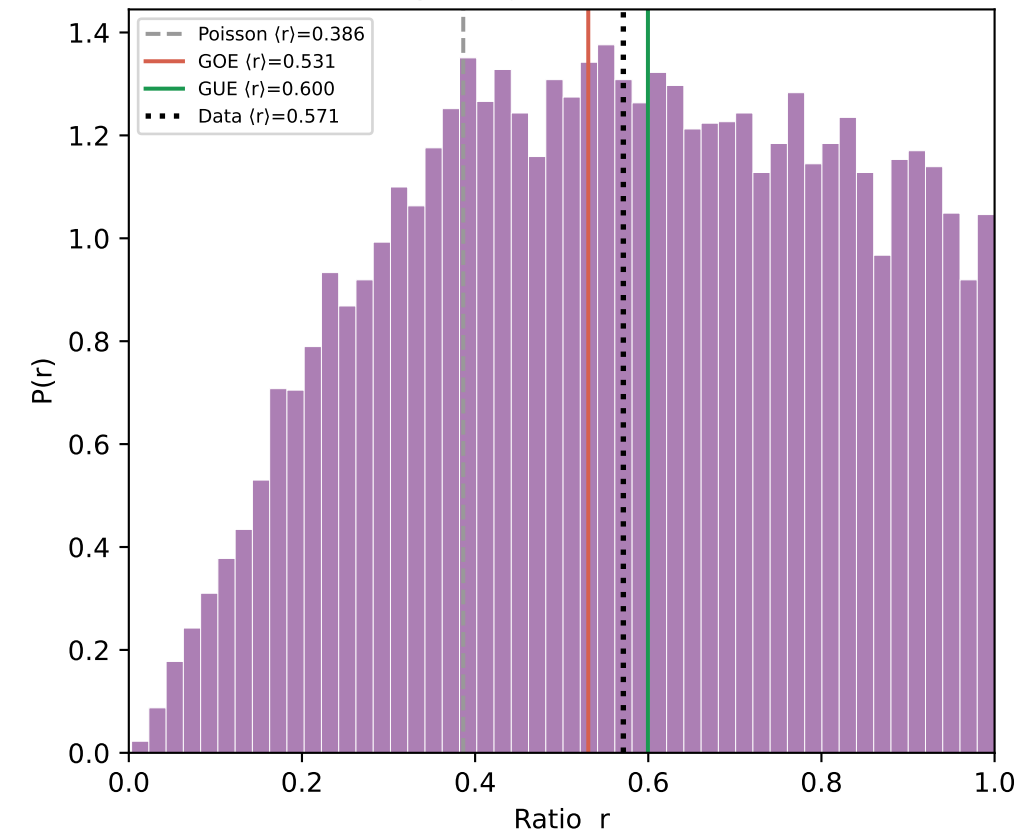
(f) Spacing ratio — Herm L
