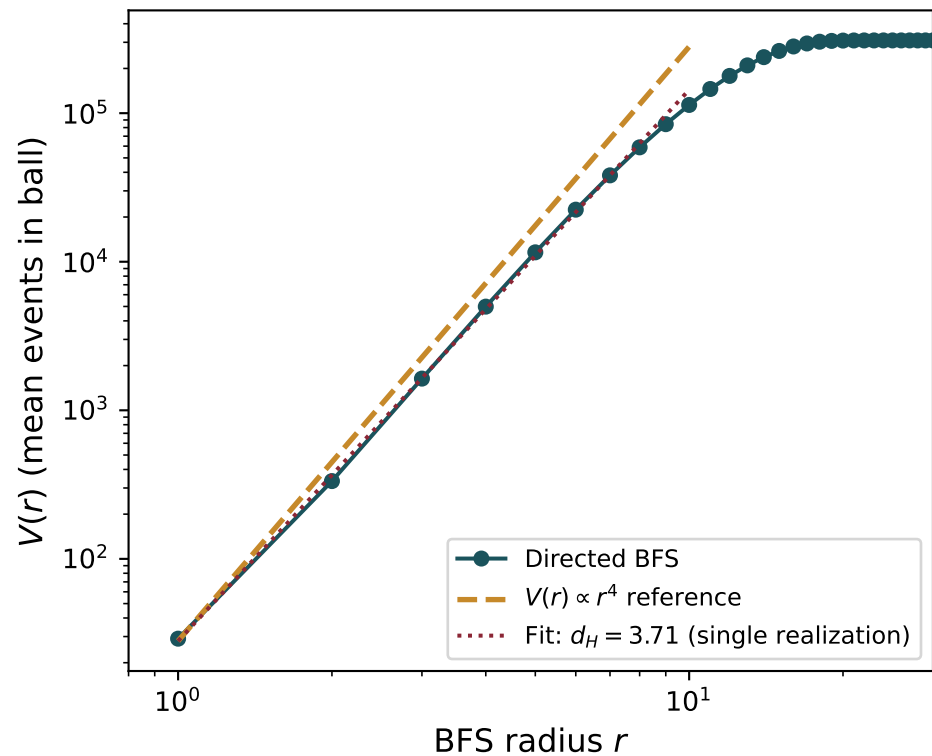
Directed BFS Volume Growth ( N = 10^7 )
