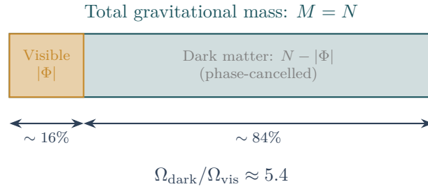
Figure 17.2: Mass decomposition. The total gravitational mass M = N of a prism splits into a visible (phase-coherent) component |\Phi| and a dark (phase-cancelled) component N - |\Phi| . For large- N prisms, |\Phi|/N \rightarrow 0 by the CLT: they are gravitationally massive but electromagnetically invisible.
