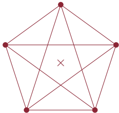
4-Simplex ( K_5 )
