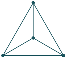
3-Simplex ( K_4 )
