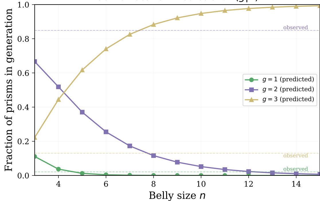
Combinatorial Prediction: P(g|n)
