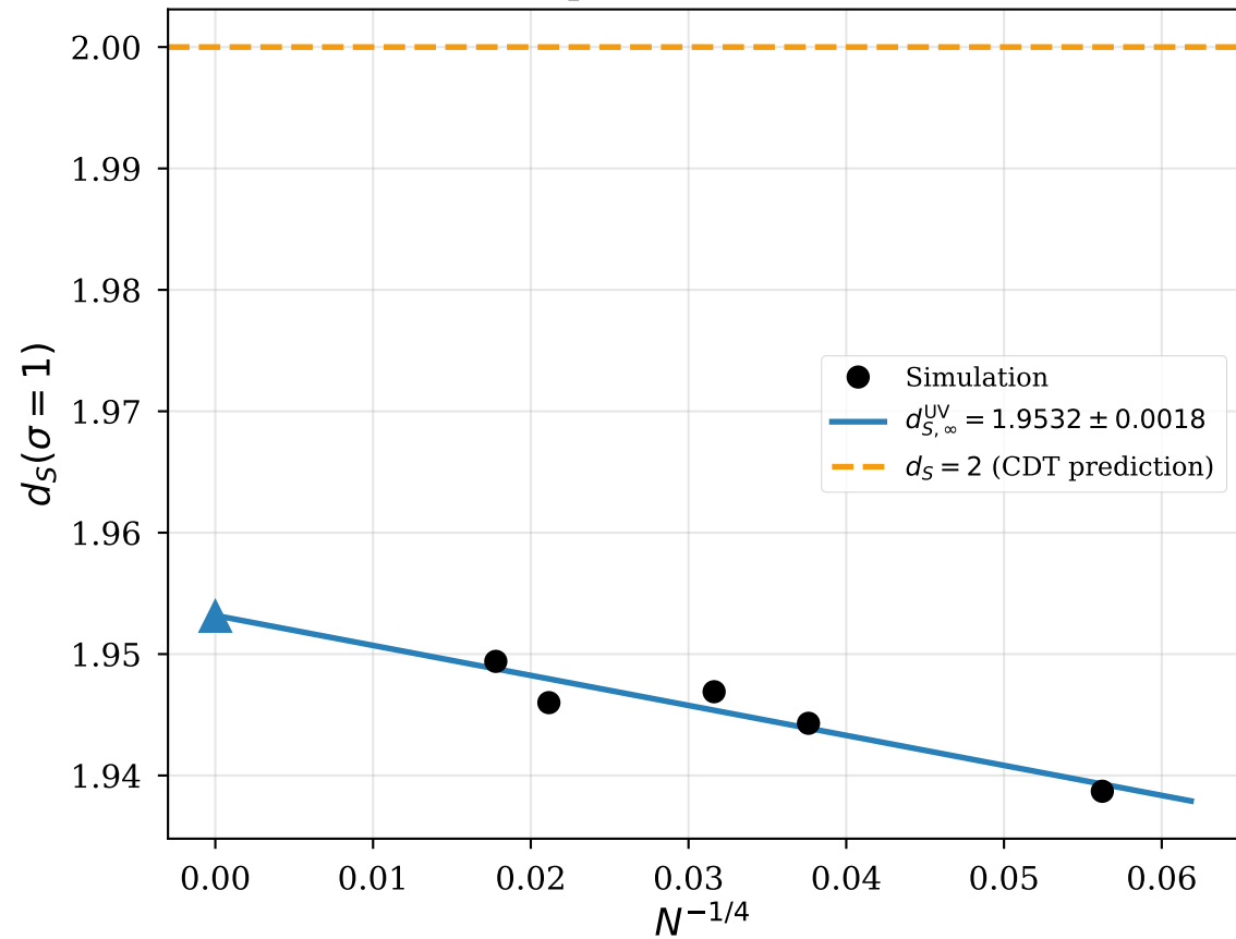
UV Spectral Dimension
