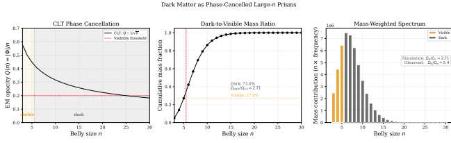
FIG. 6. Dark matter as phase-cancelled large- n prisms. Left: CLT opacity Q \sim 1/\sqrt{n} . Centre: cumulative mass fraction showing dark/visible boundary. Right: mass-weighted histogram. \Omega_{\text{energy}} = 1/Q_{\text{topo}} - 1 = 4.25 (self-energy decomposition).
