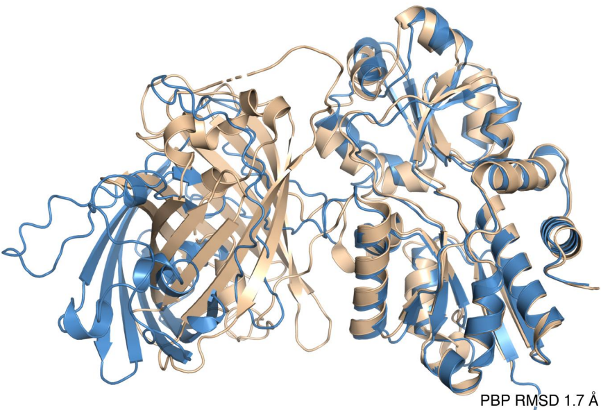
d ESMFold prediction vs crystal
