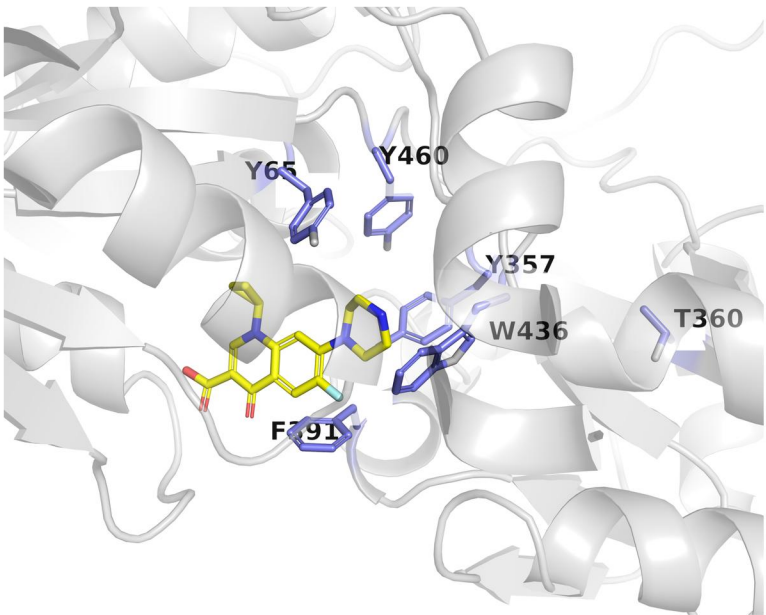
d ESMFold prediction vs crystal
