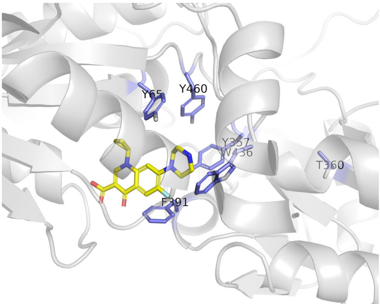
d ESMFold prediction vs crystal
