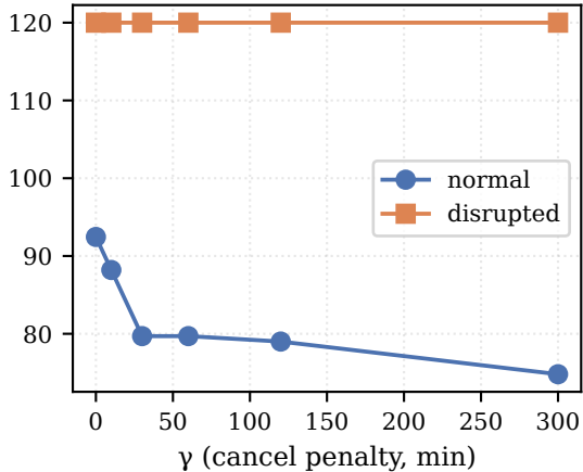
\gamma sensitivity
