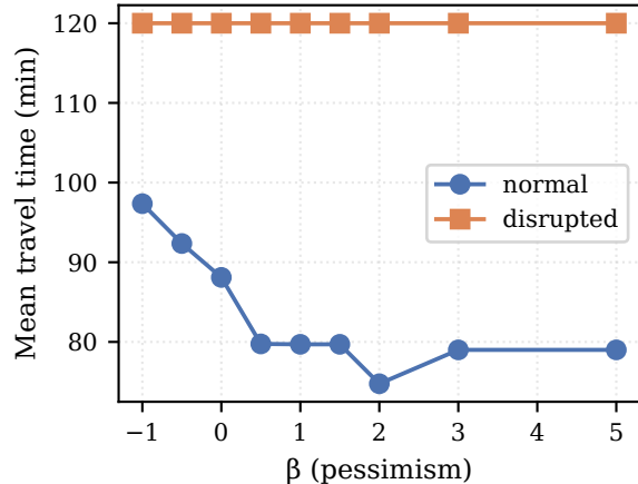
\beta sensitivity
