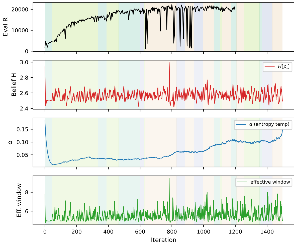
BAPR on Ant-v2 discrete-mode (seed 2): true mode (background) + return + BOCD signals
