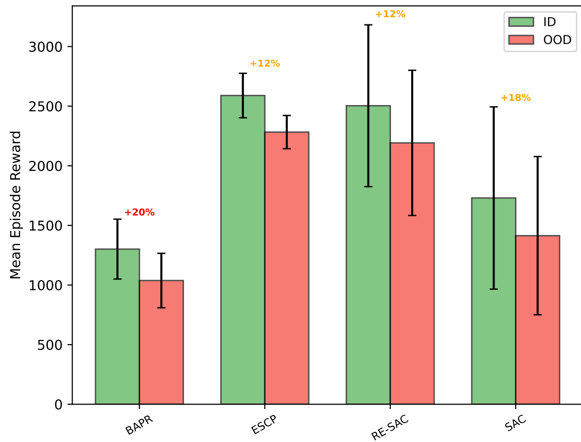
HalfCheetah
