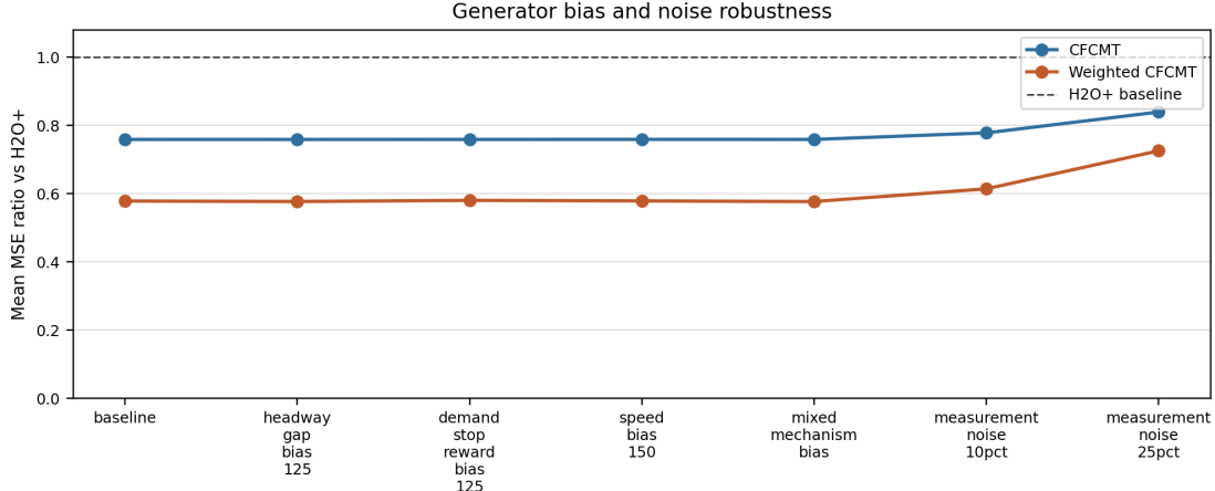
Figure 4: Generator-bias and measurement-noise robustness under strict leave-one-city-out evaluation.
