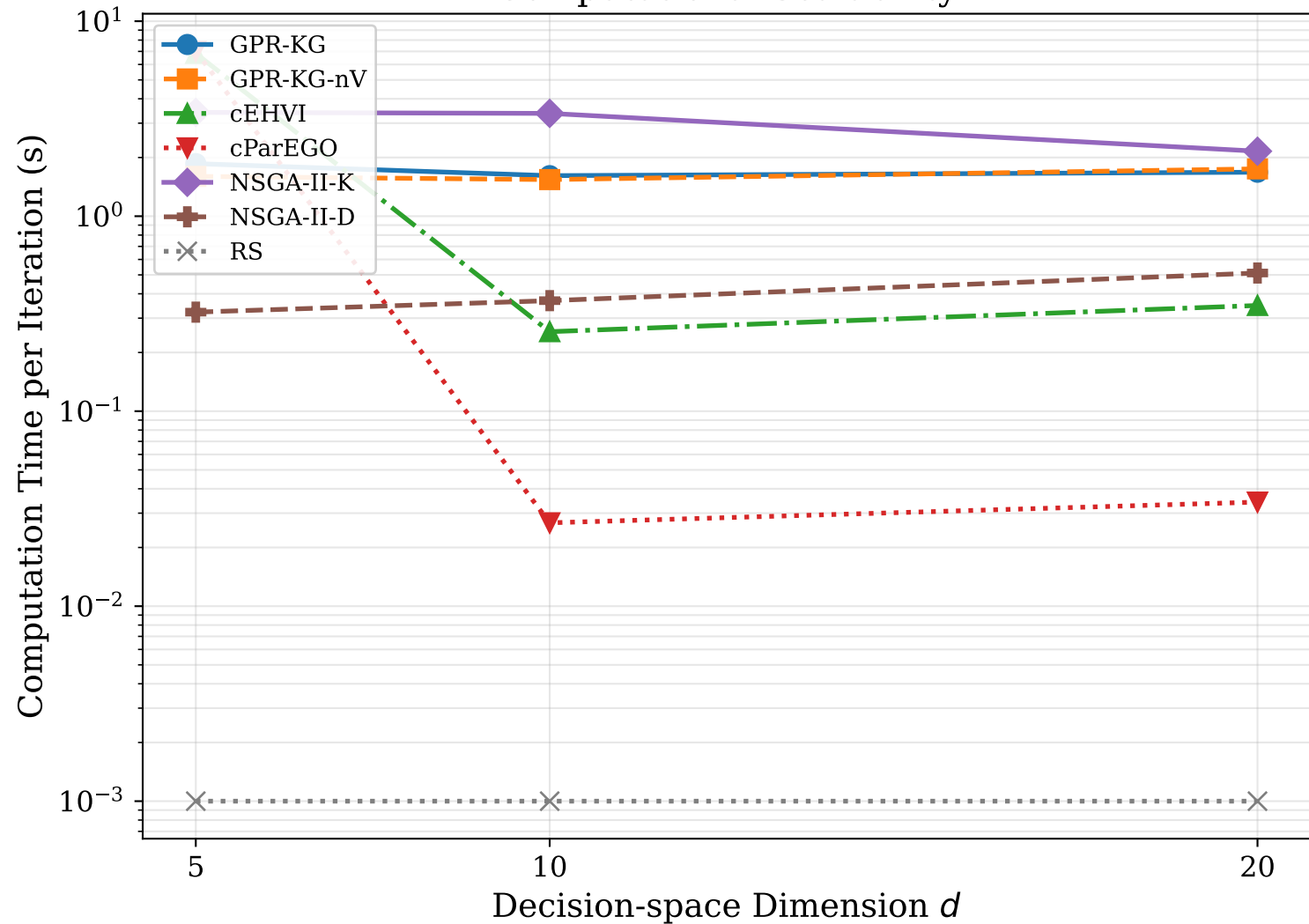
Computational Scalability
