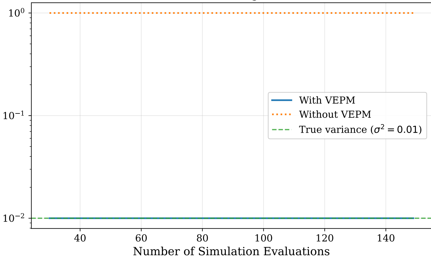
VEPM Variance Convergence on RZDT1
