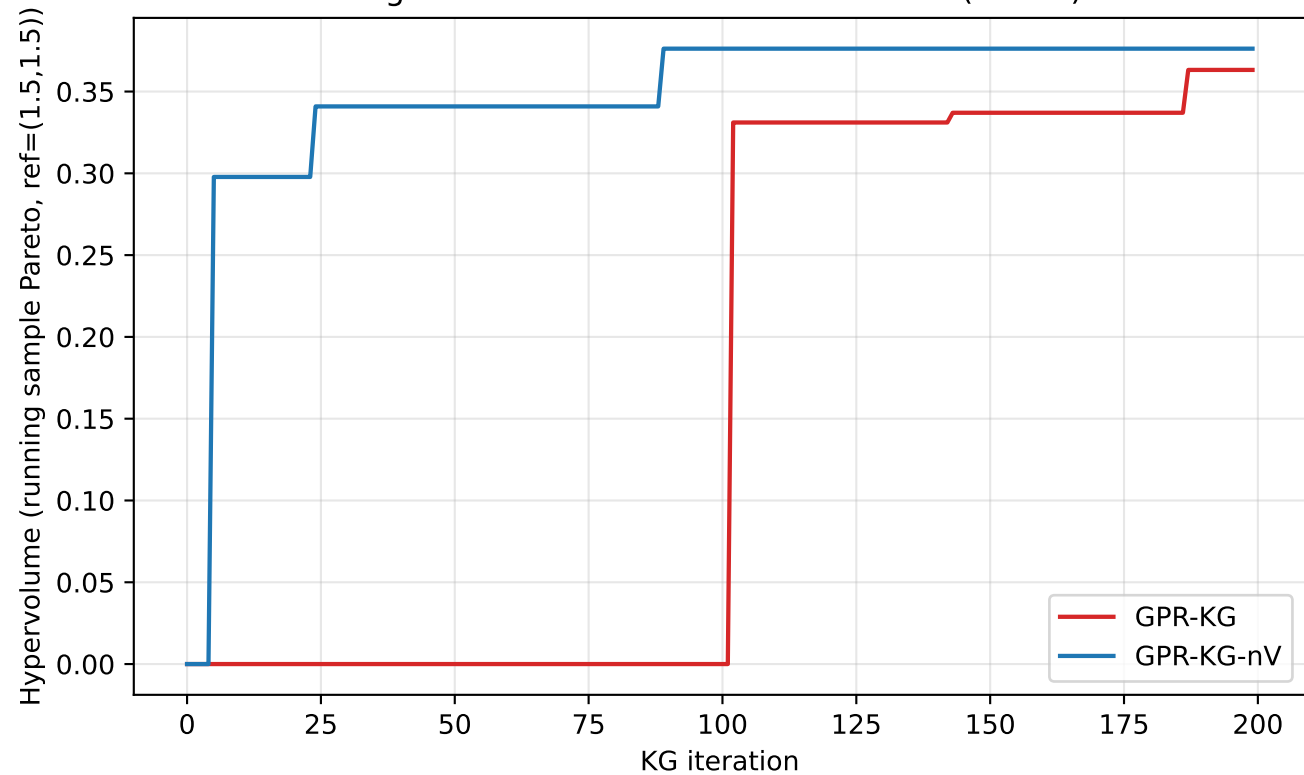
ingolstadt21 Phase 2: HV vs iteration ( \tau=1.0 )
