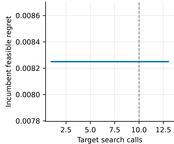
FactorShock
