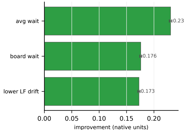
d Native real-demand score
