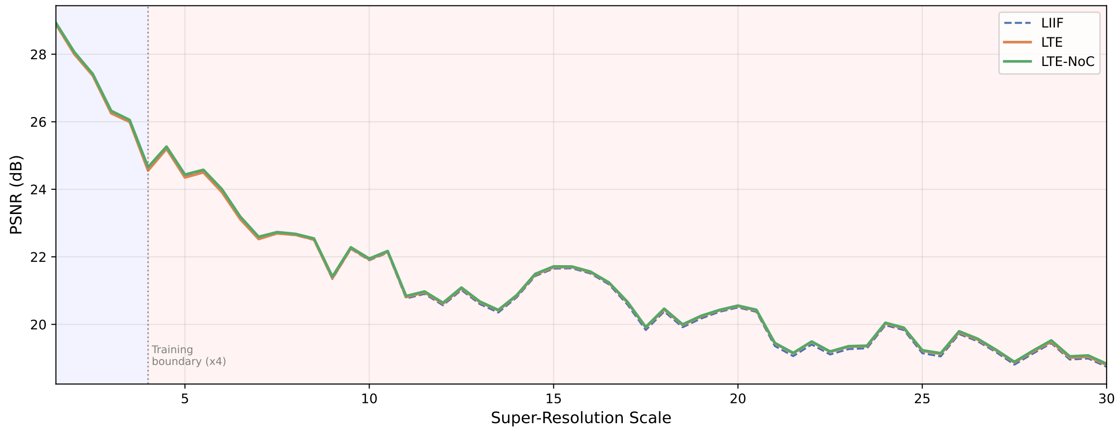
Continuous Scale PSNR — BSD100
