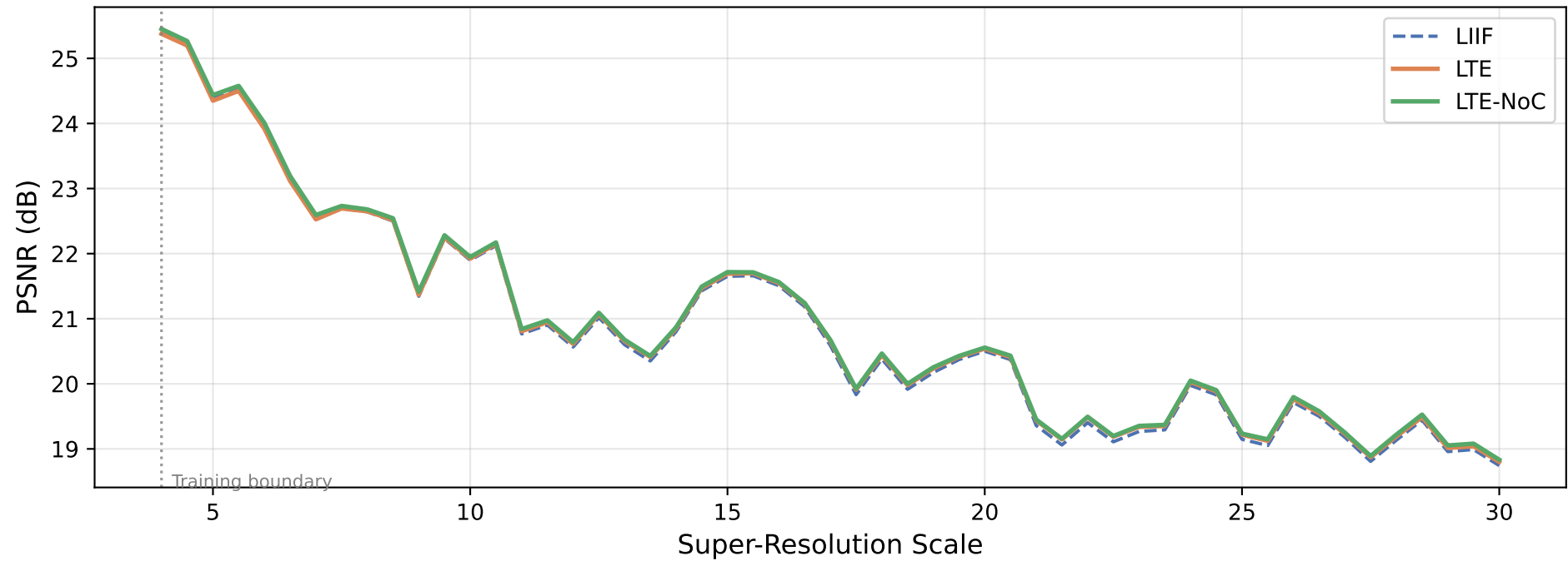
OOD Generalization: Continuous Scale PSNR — BSD100
