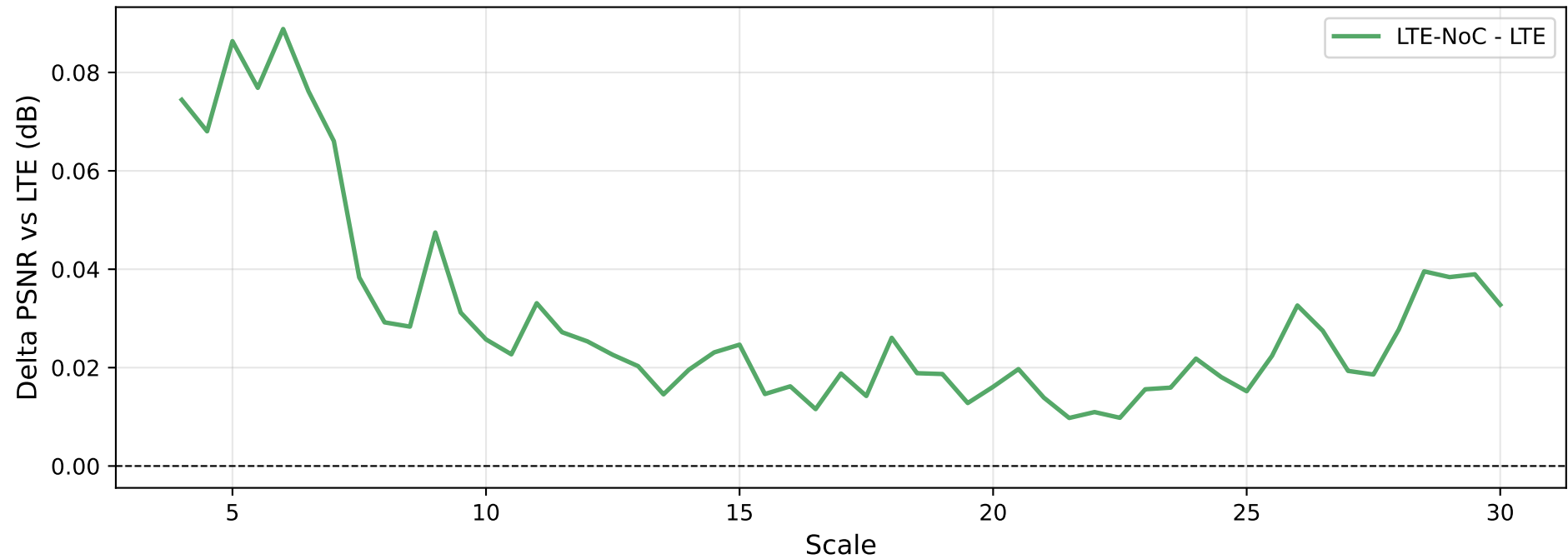
PSNR Difference: LTE-NoC minus LTE — OOD region
