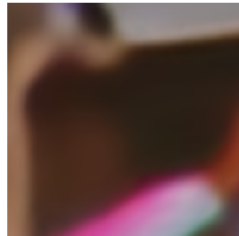
SC-INR 28.2289 dB
