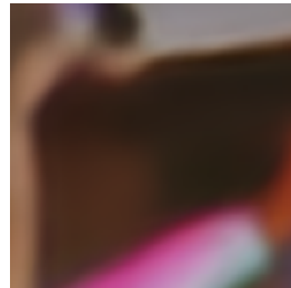
SC-INR+PhiZ 28.7003 dB
