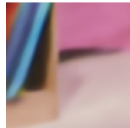
SC-INR+PhiZ 29.7766 dB
