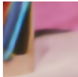
LTE 29.3283 dB
