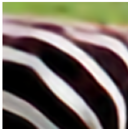
LTE 20.6902 dB
