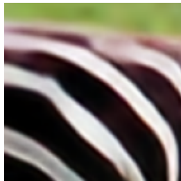
SC-INR 21.1927 dB
