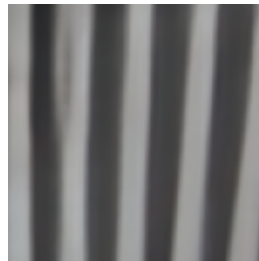
SC-INR 13.4222 dB
