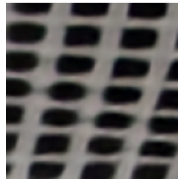
SC-INR 21.4880 dB
