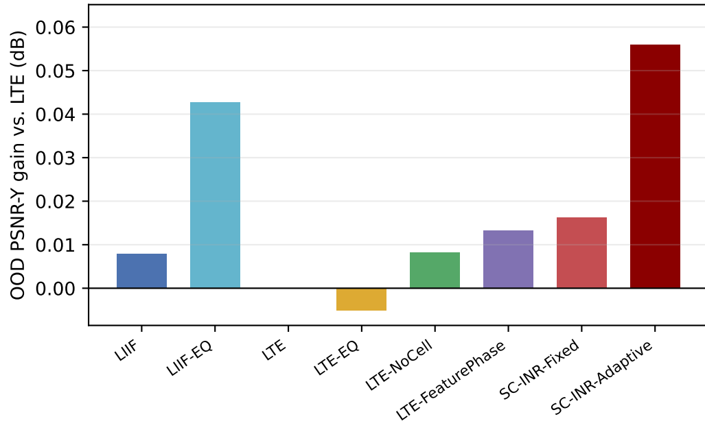
BSD100
