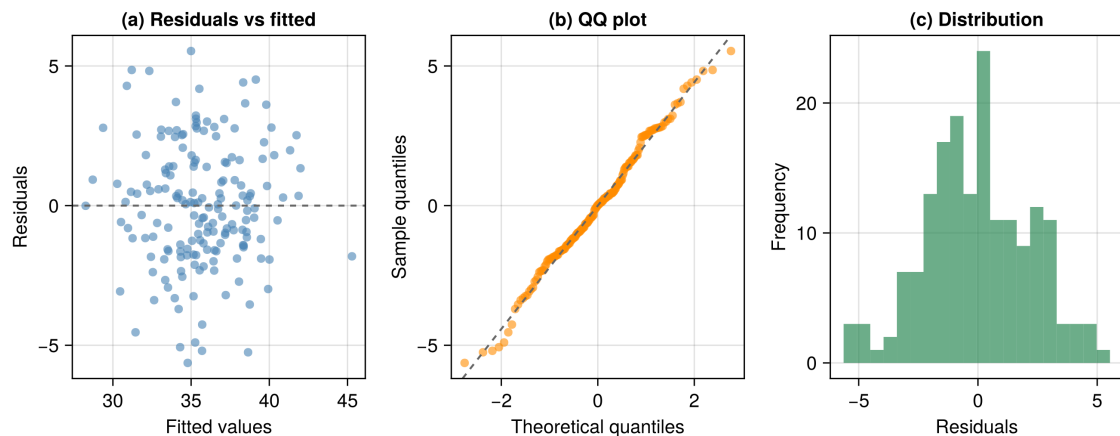
Figure 8.1: Residual diagnostics for model m3.
