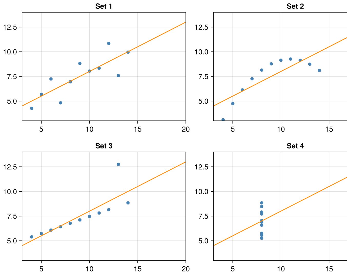
Figure 7.4: The Anscombe quartet: four data sets with the same summary statistics and the same least-squares line.
