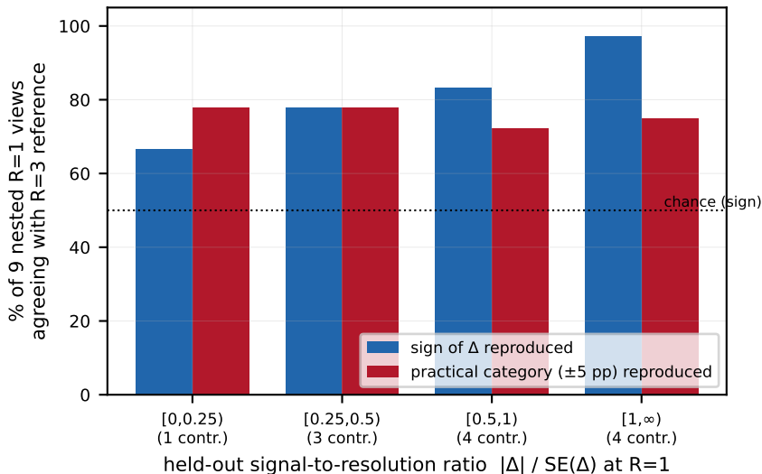
Fig 5 Calibration predicts sign reliability, but NOT practical-category reliability
