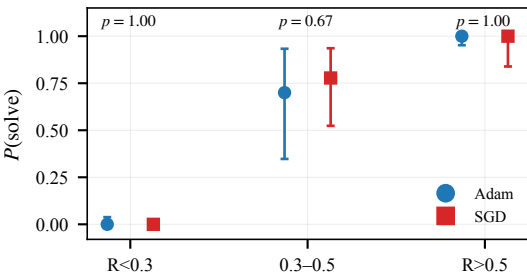
(b) same curve for both optimisers ( a = 1.25 , n = 180 each) Fisher exact, two-sided
