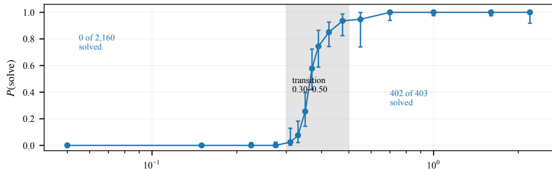
(b) same curve for both optimisers ( a = 1.25 , n = 180 each) Fisher exact, two-sided
