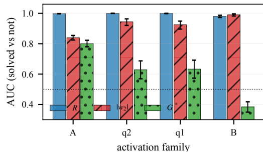
(c) R beats both factors — except family B ( \beta = 1 )
