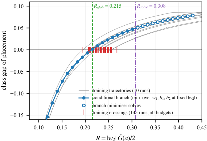
(a) conditional branch and training, a = 1.30
