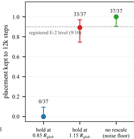
(b) intervening on |w_2| after placement
