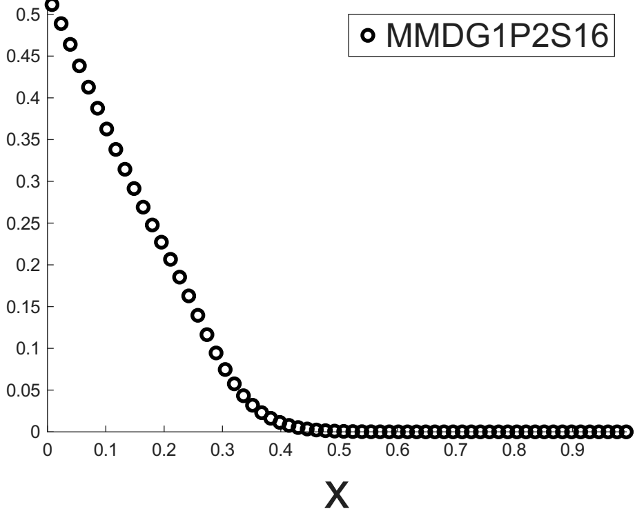
Radiation with MMDG1P2S16 at t = 0.40
