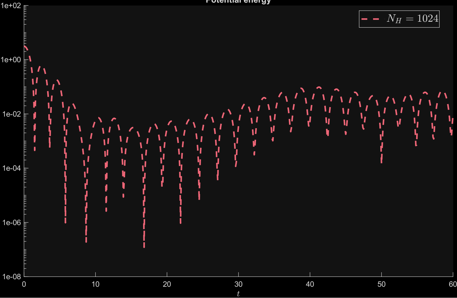
Potential energy
